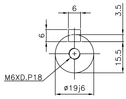
SECTION "X-X"
